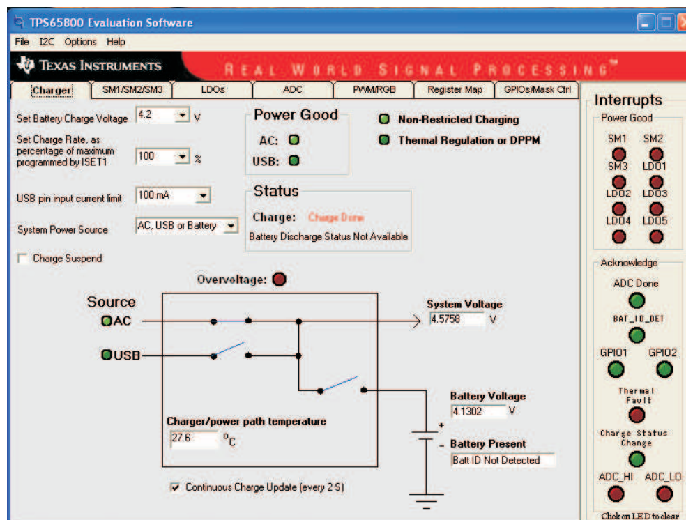
Figure 3. Charger Section
