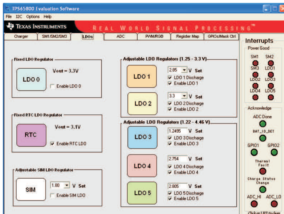
Figure 5. LDO Section
